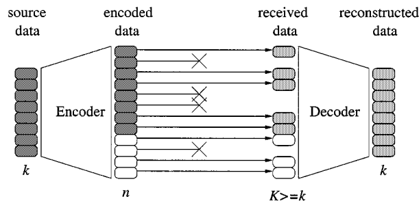
Fig. 12. Channel coding/decoding operation.
