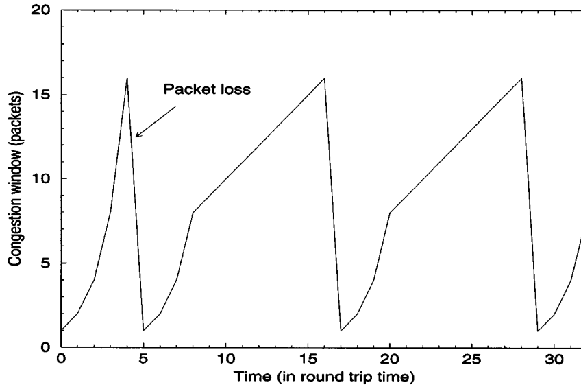
Fig. 4. Congestion window behavior under window-based control.
