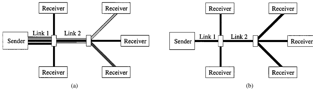
Fig. 2. (a) Unicast video distribution using multiple point-to-point connections. (b) Multicast video distribution using point-to-multipoint transmission.
