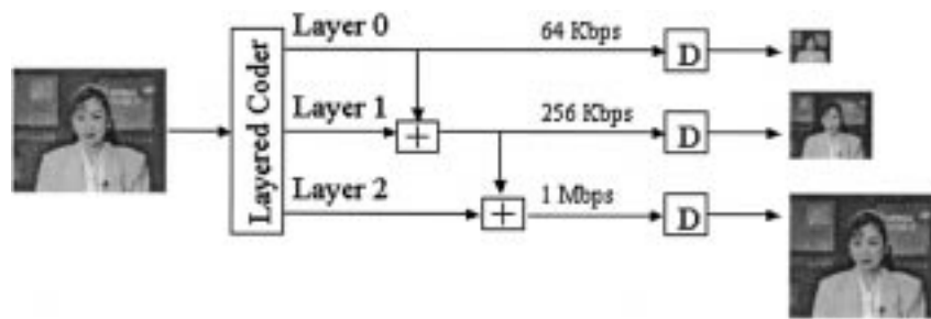
Fig. 7. Layered video encoding/decoding. D denotes the decoder.
