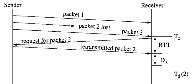
Fig. 15. Timing diagram for receiver-based control.
