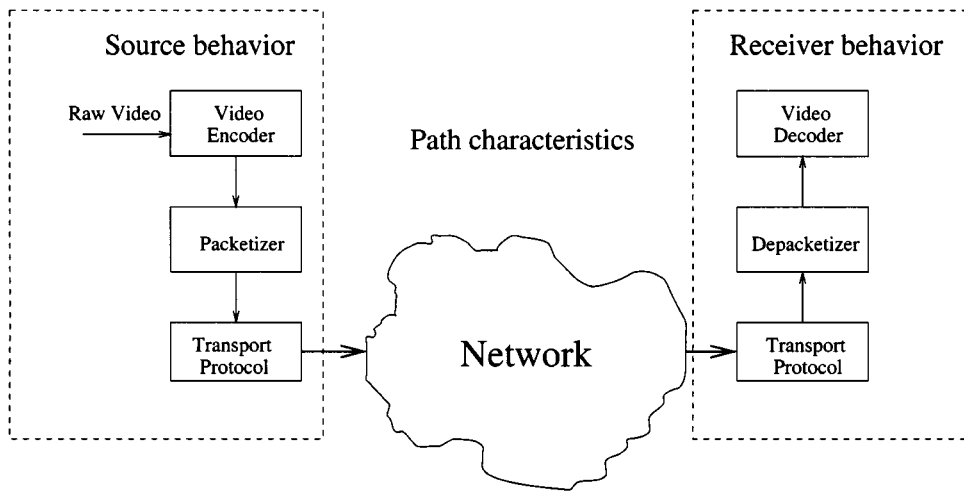
Fig. 18. Factors that have impact on the video presentation quality: source behavior, path characteristics, and receiver behavior.
