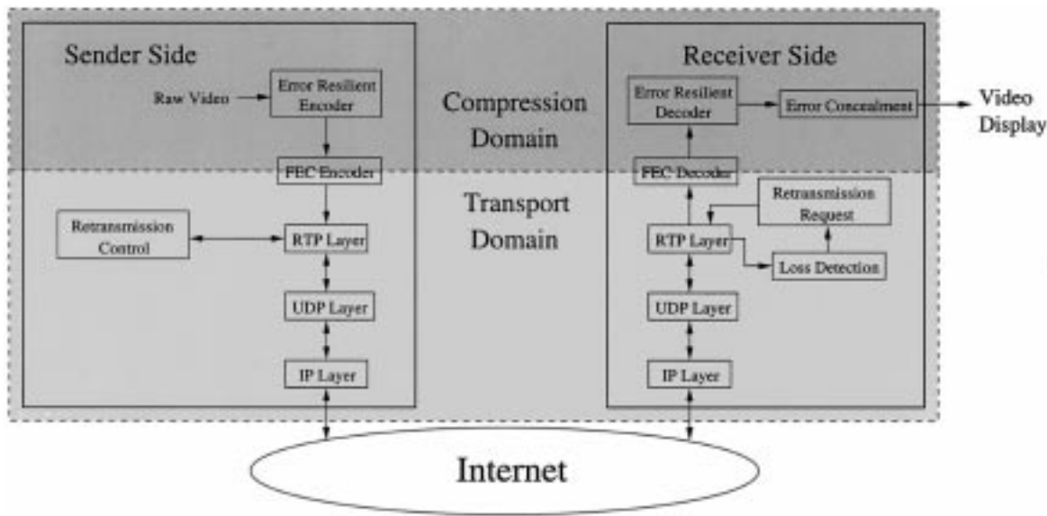
Fig. 11. Architecture for error-control mechanisms.
