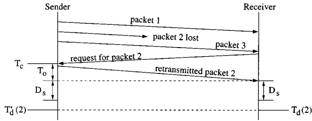
Fig. 16. Timing diagram for sender-based control.
