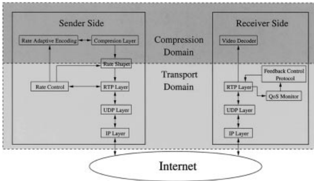
Fig. 3. Layered architecture for transporting real-time video.
