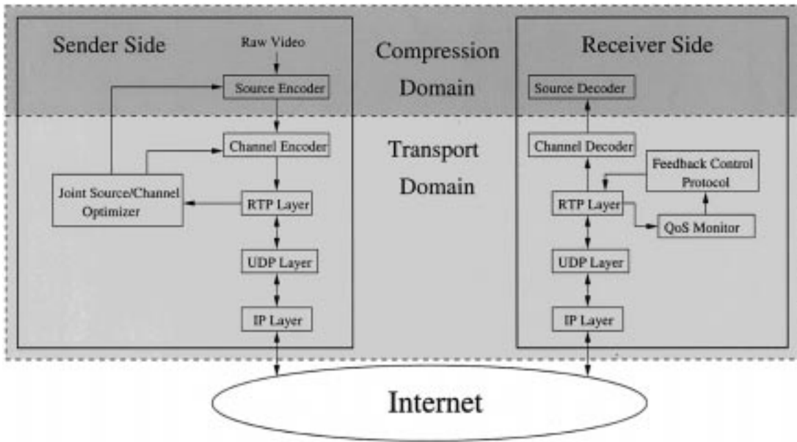
Fig. 14. Architecture for joint source/channel coding.
