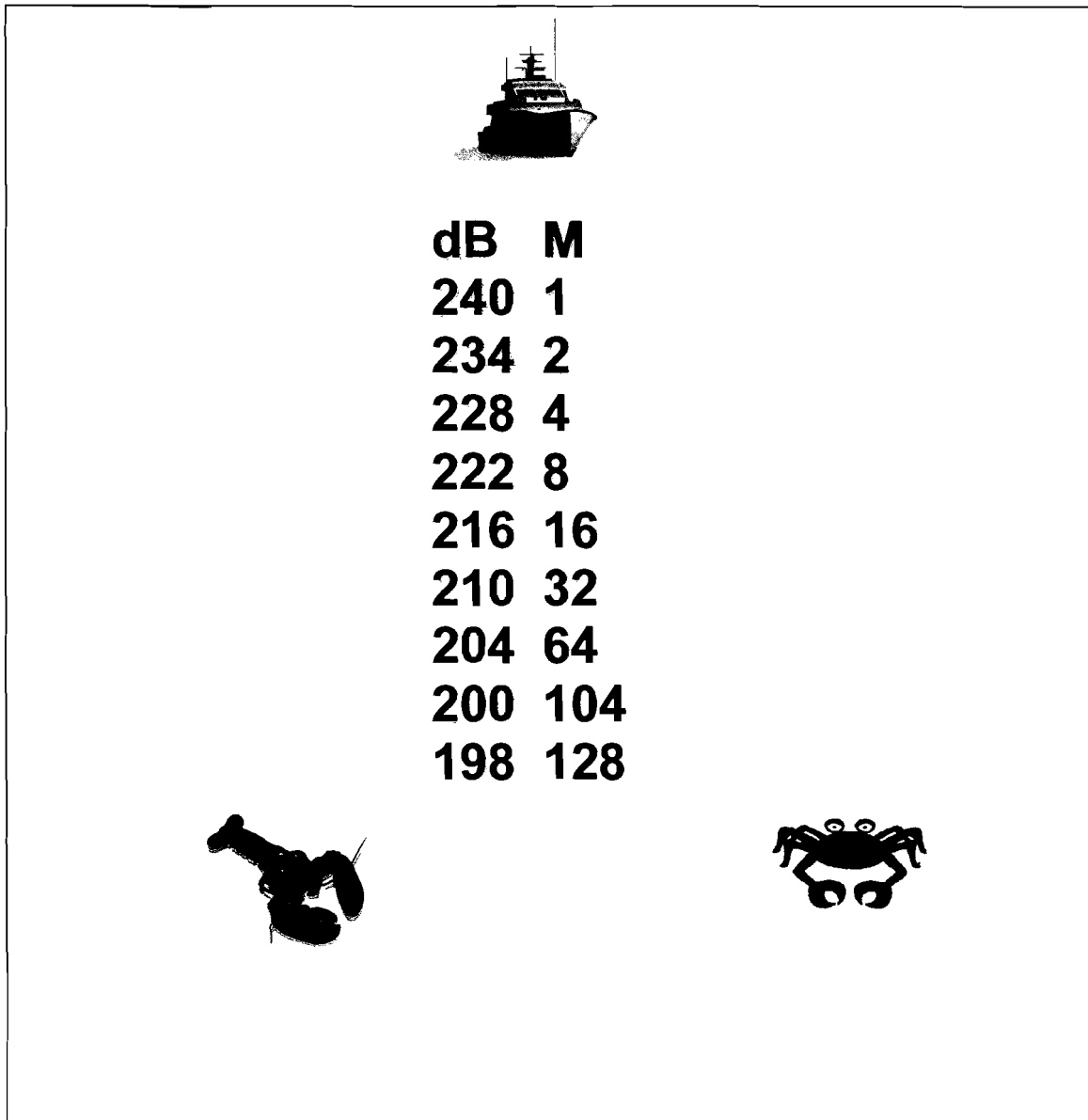
Figure 34. Hypothetical distances for sound travel down into the water column assuming spherical spreading.
