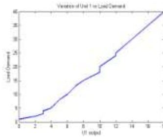
Fig 4. Variation of U1 output vs Load demand
