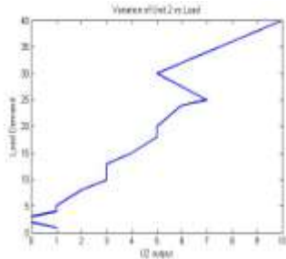
Fig 5. Variation of U2 output vs Load demand
