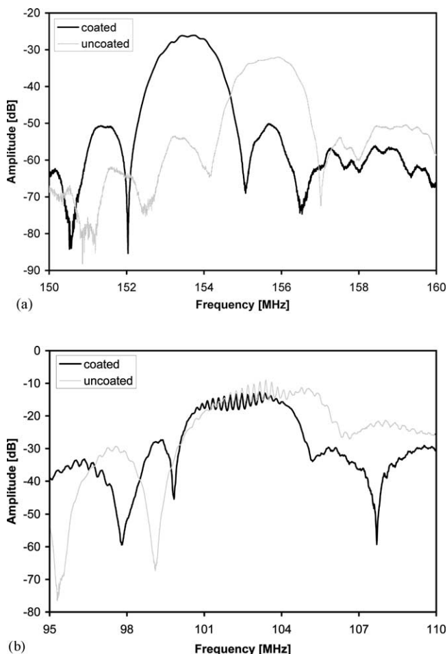
Fig. 3. (a) Transmission spectrum of the quartz 155 MHz (Q155) device where amplitude is plotted as a function of frequency before and after the device is coated with 0.87 \mu\text{m} of Novolac; (b) transmission spectrum of the \text{LiTaO}_3 104 MHz (LT104) device where amplitude is plotted as a function of frequency before and after the device is coated with 1.75 \mu\text{m} of Novolac.
