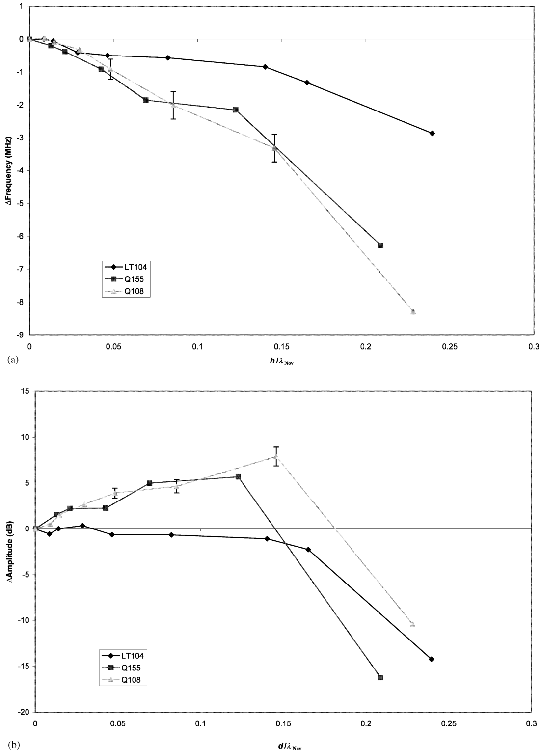
Fig. 4. (a) Frequency and (b) amplitude change as a function of the normalised thickness ( h/\lambda_{Nov} ), where h is the Novolac thickness and \lambda_{Nov} the acoustic wavelength inside the layer for the LiTO 3 104 MHz (LT104), quartz 155 MHz (Q155) and quartz 108 MHz (Q108) devices.
