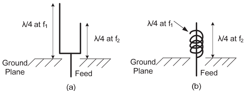
Fig. 4. (a) Two monopole antennas for dual-band operation (b) A helical antenna resonating at the frequency f_1 and a monopole antenna resonating at the frequency f_2 for dual-band operation
