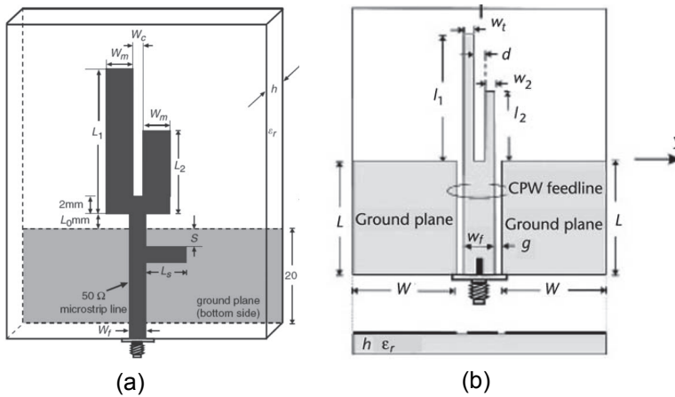
Fig. 8. (a) A microstrip fed dual-band printed monopole antenna (Chen et al., 2001) (b) A coplanar waveguide (CPW) fed dual-band printed monopole antenna (Chen & Chen, 2004)
