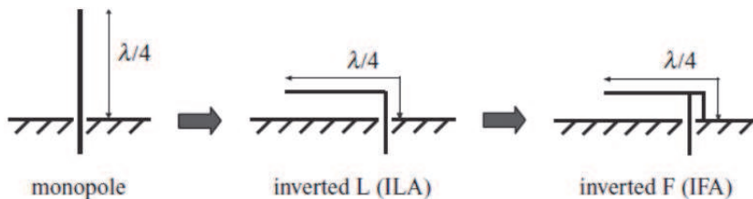
Fig. 9. Modification steps of IFA from monopole antenna (Huang & Boyle, 2008)
