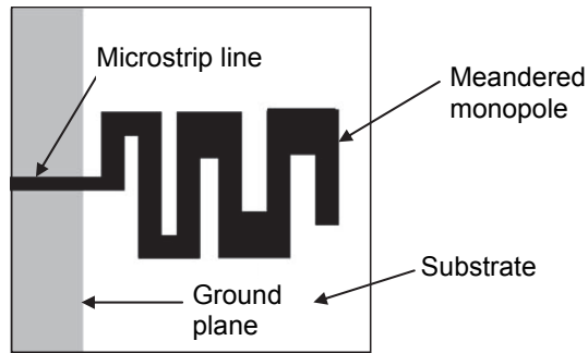
Fig. 13. A meandered printed monopole antenna
