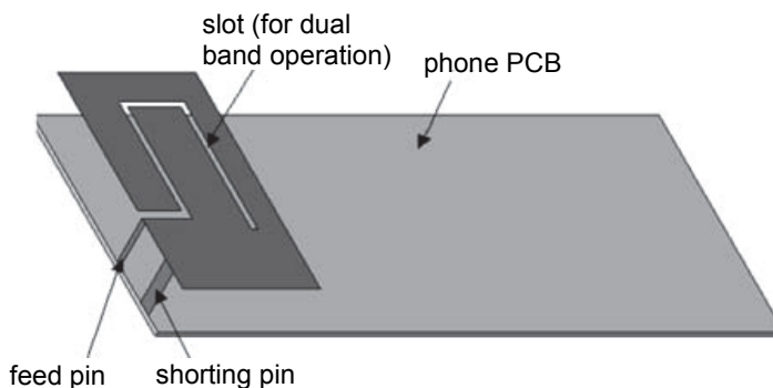
Fig. 11. A dual-band PIFA structure (Boyle, 2008)
