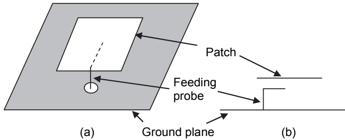
Fig. 18. (a) Isometric and (b) side views of the suspended plate antenna
