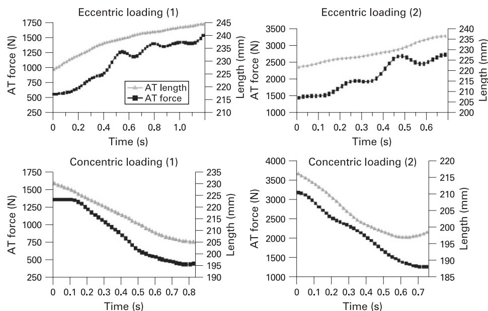
Figure 4 Force characteristics for eccentric and concentric loading of the AT. In eccentric loading the AT is subject to repeated unloading and loading in a sinusoidal-type pattern. In concentric loading, this additional loading and unloading are largely absent. Typical examples are shown for one woman (subject 1) and one man (subject 2). Eccentric loading is shown in the top two graphs and concentric loading in the bottom two graphs.
