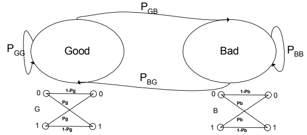
Figure 2. Gilbert-Elliott channel model
