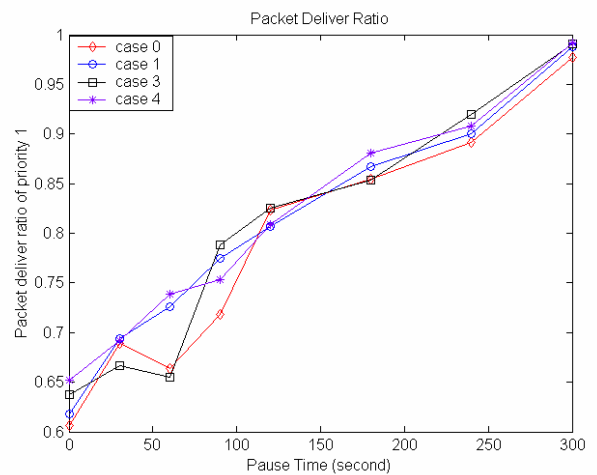
Figure 10.d. Packet delivery ratio of Priority 1 service
