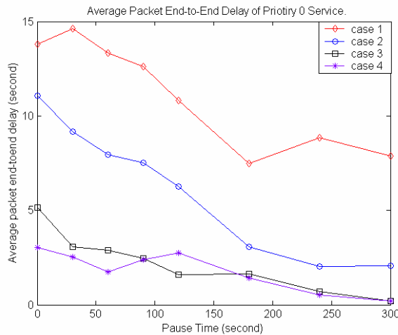
Figure 10.a. Average end-to-end delay of priority 0 service
