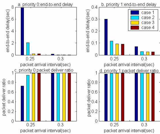
Figure 9. Simulation results with different packet arrival rates.
