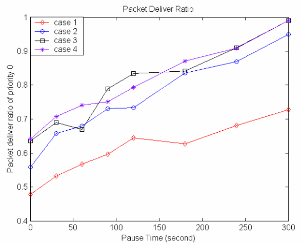
Figure 10.c. Packet delivery ratio of Priority 0 service
