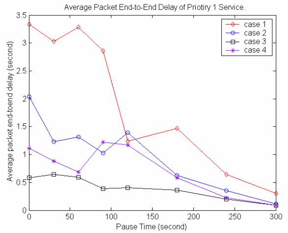
Figure 10.b Average end-to-end delay of priority 1 service
