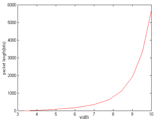
Figure 3. Optimal packet length vs SNR( \gamma ), h=128
