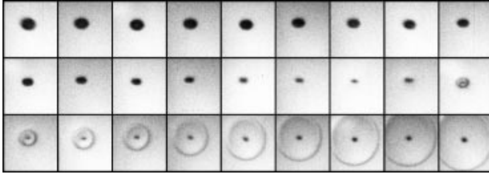
Figure 3. A spherically symmetric shock wave emitted by a laser-generated bubble upon first collapse taken at 20.8 million frames per second with the arrangement depicted in figure 1. The frame size is 1.5 \times 1.8 \text{ mm}^2 and the exposure time is ca. 5 ns.
