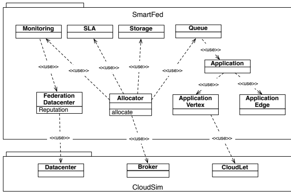
Figure 1: Main entities of SmartFed
