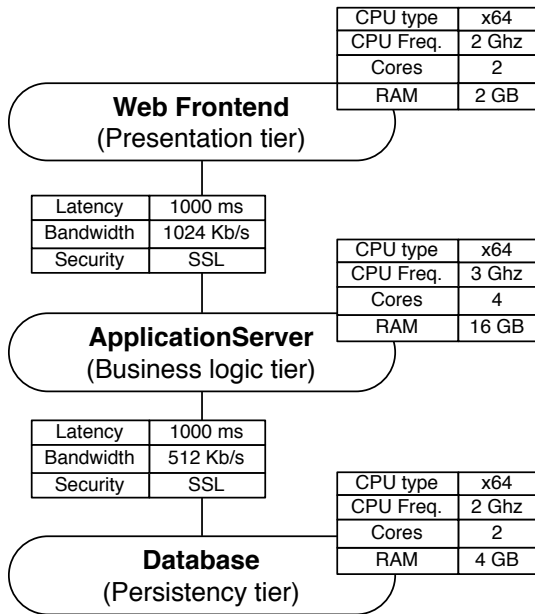
Figure 3: The 3-tier application used in the simulation
