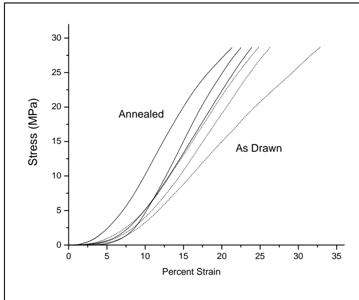
Figure 26. Cooled compression tests of cylindrical IM 800A. T = -75\text{ }^{\circ}\text{C} .
