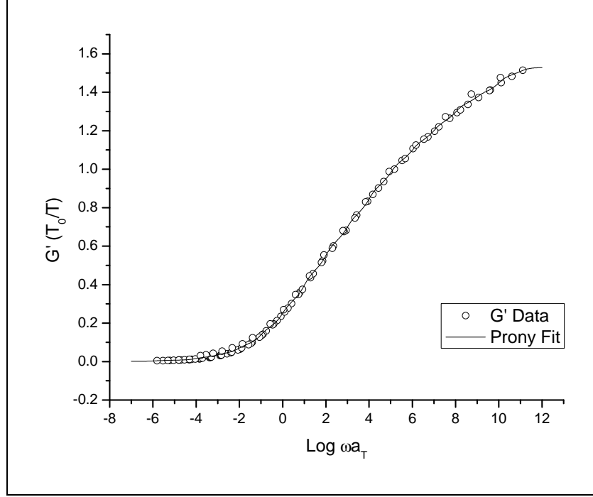
Figure 19. Prony fit of rheometer shear storage modulus data, T_0 = -61 °C.
