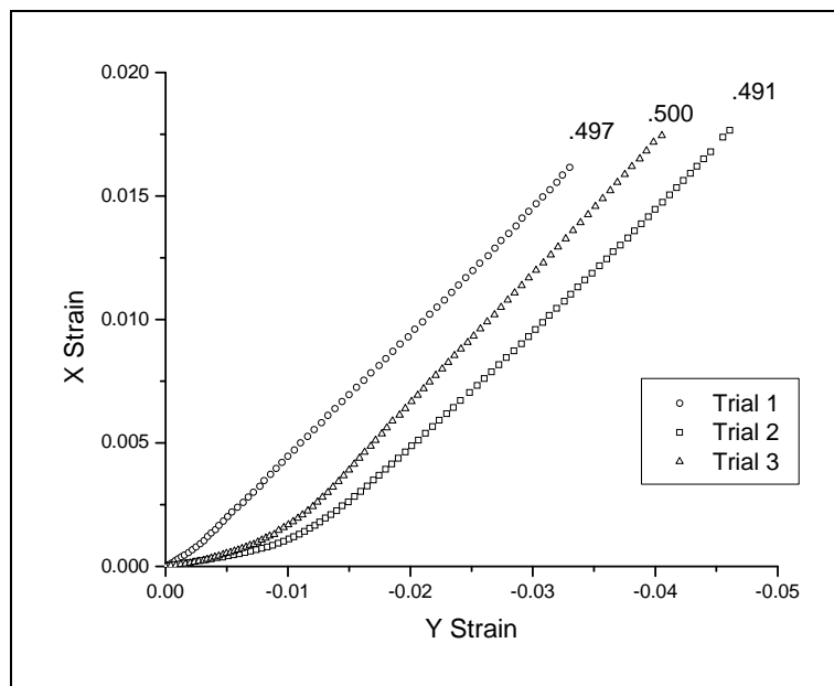
Figure 24. Perpendicular (X) strain vs. parallel (Y) strain during compression for IM 800A TPU as determined by VIC analysis. T = 25\text{ }^{\circ}\text{C} .
