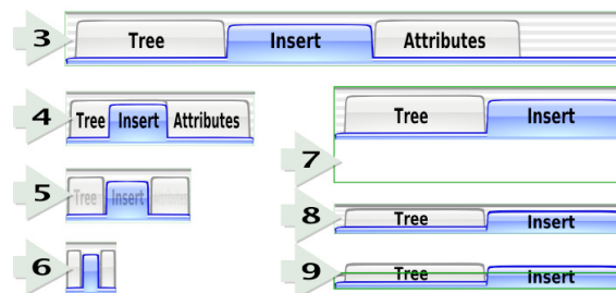
Figure 6: Scenario, continued: examples 3, 4, 5 and 6 describe the behavior for smaller and larger widths, whereas 7, 8 and 9 specify the vertical behavior.
