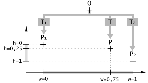
Figure 8: Geometrical interpretation of orthogonal interpolation. Here, an intermediate transformation T is applied to a point O , with T = I_{((0,0), T_1), ((1,1), T_2)}^{orth}(0.75, 0.25) .
