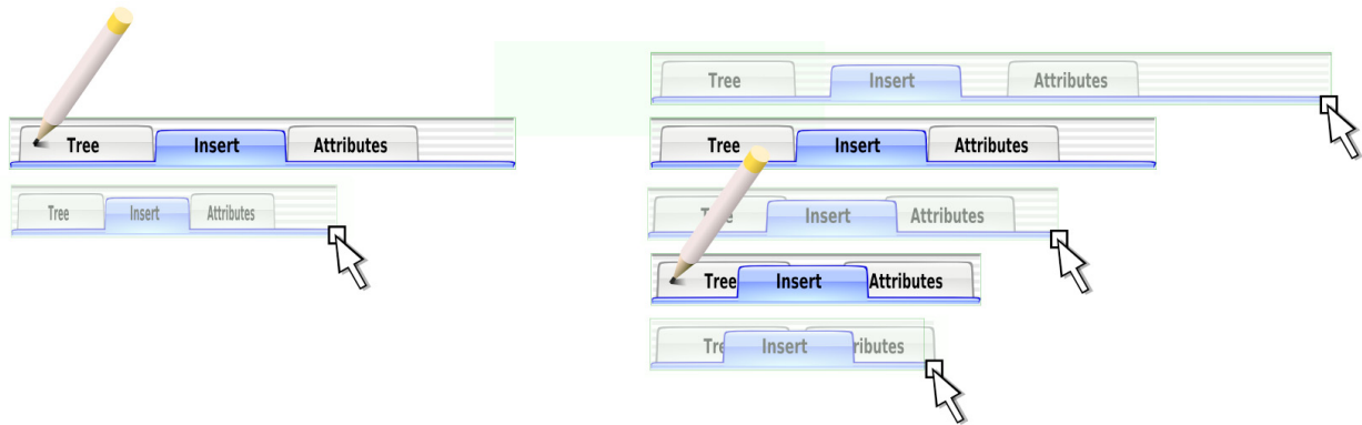
Figure 5: A possible scenario: on the top left, the graphic designer draws a graphical object and sees how it behaves when naively scaled (1). She then decides to draw a second example to specify another way of shrinking the object (2). The new resizing behavior can now be tested to see how it behaves between and outside the examples.
