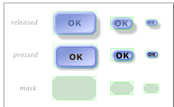
Figure 4: The SVG specification of Figure 3c, with the three button parts and their bounding boxes.
