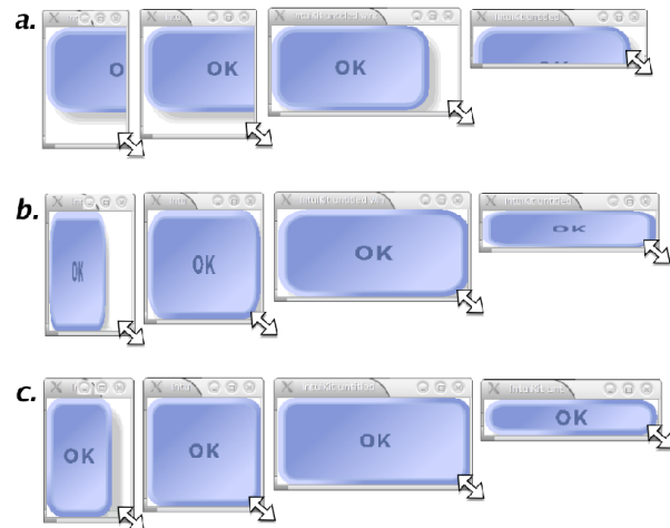
Figure 3: Three resizing strategies for a vector graphics button: fixed layout (a), naive scaling (b) and commonly expected resizing (c).
