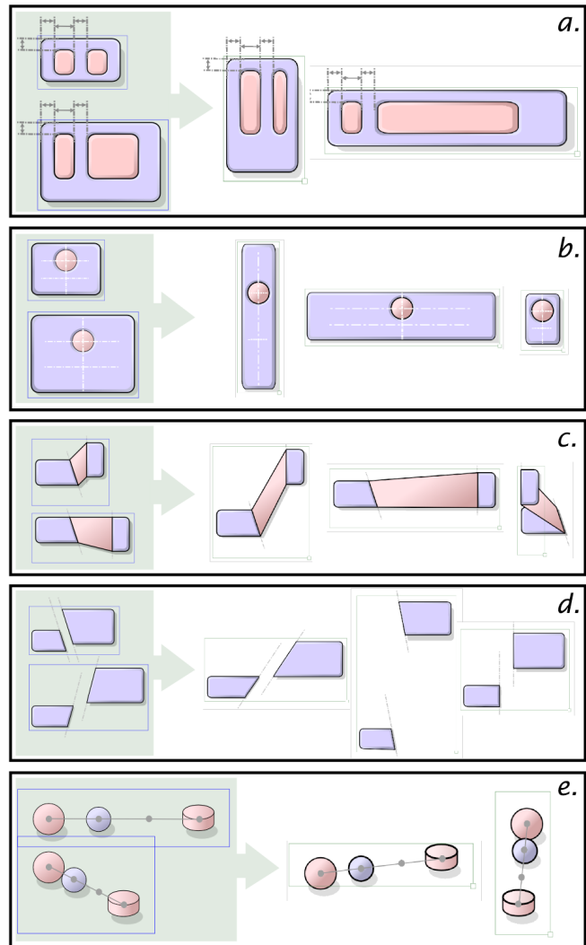
Figure 10: Conservative properties illustrated: a. preservation of projected algebraic measures, b. preservation of ratios, c. preservation of coincident vertices, d. preservation of parallelism, e. preservation of affine combinations.
