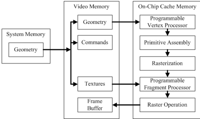
Fig. 1. The programmable graphics pipeline
