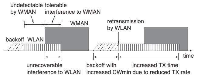
FIGURE 2. Responses of WMAN and WLAN to inter-system interference.
