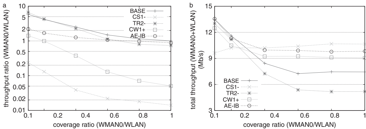
FIGURE 11. Performance comparison of several approaches with different values of the WLAN's coverage. (a) Throughput ratio ( \gamma_{\text{ratio}} ) and (b) total throughput ( \eta_{\text{eff}} ).
