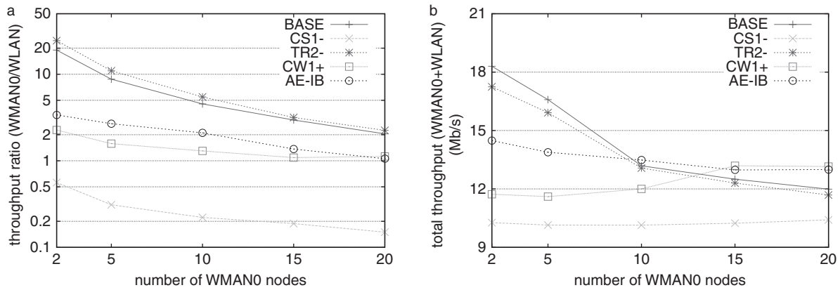
FIGURE 12. Performance comparison of several approaches with different values of the number of WMAN nodes. (a) Throughput ratio ( \gamma_{\text{ratio}} ) and (b) total throughput ( \eta_{\text{eff}} ).
