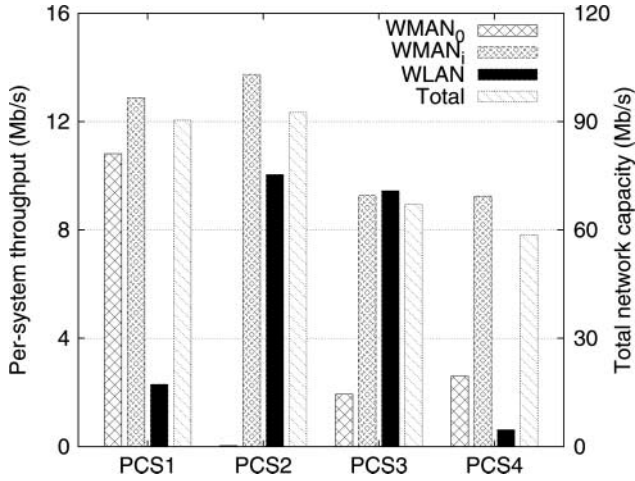
FIGURE 3. Per-system throughput and aggregate network capacity for four cases with different values of the CSTH.
