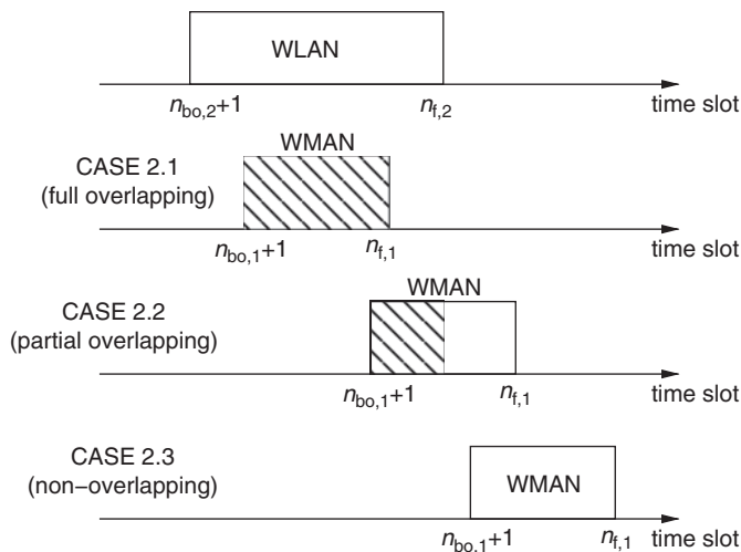
FIGURE 4. Three sub-cases of inter-system interference when n_{\text{bo},1} \geq n_{\text{bo},2} .
