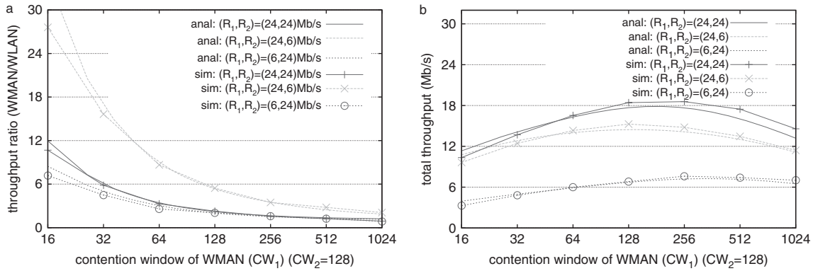
FIGURE 5. Effect of the contention window on the fairness and efficiency of channel sharing. (a) Throughput ratio ( \gamma_{\text{ratio}} ) and (b) total throughput ( \eta_{\text{eff}} ).
