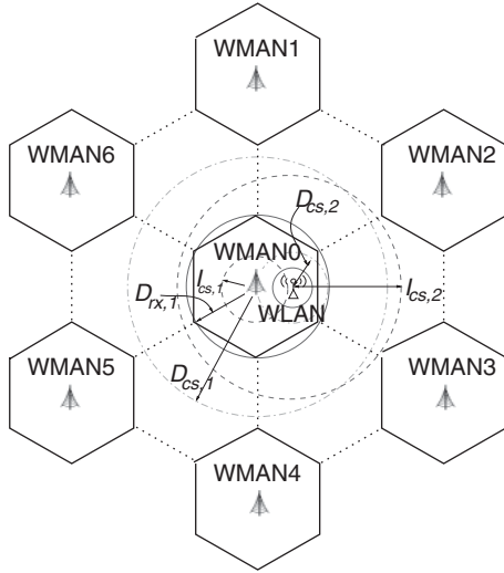
FIGURE 1. Coexistence scenario of the WMAN and the WLAN (WMANs are deployed with a frequency reuse factor of 1/3).
