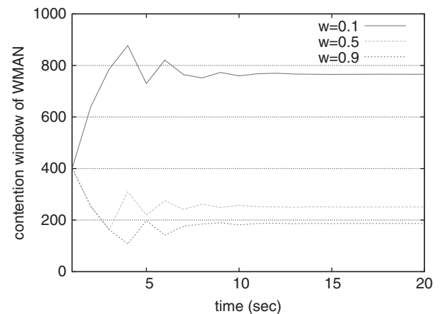
FIGURE 9. Convergence of WMAN's contention window size control according to the access etiquette scheme with different values of weight in the objective function.
