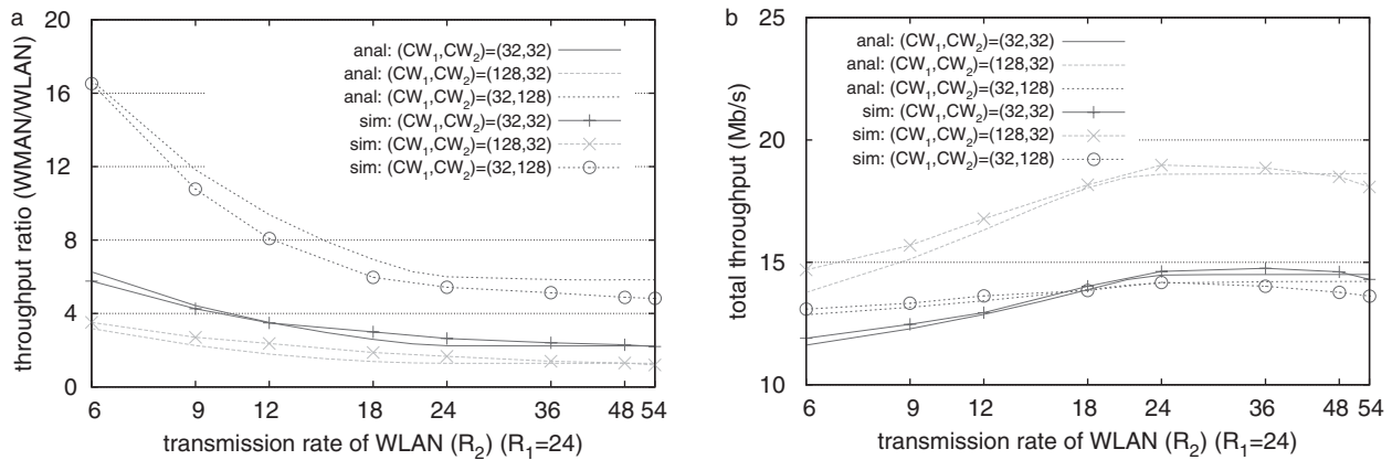
FIGURE 6. Effect of the transmission rate on the fairness and efficiency of channel sharing. (a) Throughput ratio ( \gamma_{\text{ratio}} ) and (b) total throughput ( \eta_{\text{eff}} ).
