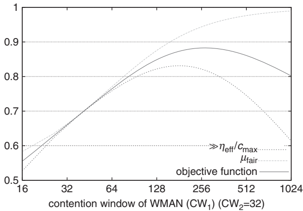
FIGURE 7. Objective function (weighted sum of \eta_{\text{eff}}/C_{\text{max}} and \mu_{\text{fair}} ) versus CW_1 .
