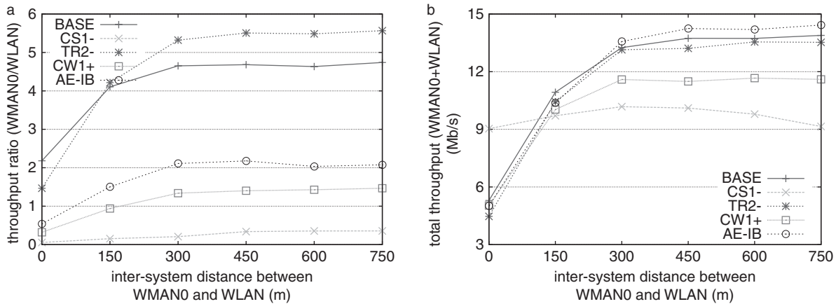
FIGURE 10. Performance comparison of several approaches with different degree of overlapping deployment between WMAN0 and the WLAN. (a) Throughput ratio ( \gamma_{\text{ratio}} ) and (b) total throughput ( \eta_{\text{eff}} ).
