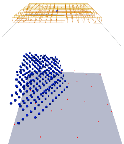
Figure 4: (a) Given: one plane and a template construction element at a small distance from the ground. (b) A fan-like structure is built (generation 506, fitness 0.0058).
