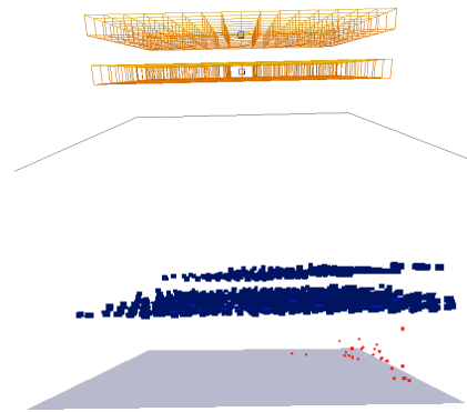
Figure 5: (a) Given are two planes. (b) A swarm of generation 314 creates “two-level flats” starting with two seed blocks at the corresponding heights (fitness 0.0122).
