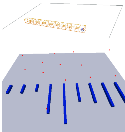
Figure 3: (a) The given 3D object that guides the evolutionary search. (b) An evolved swarm builds lines starting from any provided seed construction element (generation 15, fitness 0.0064).
