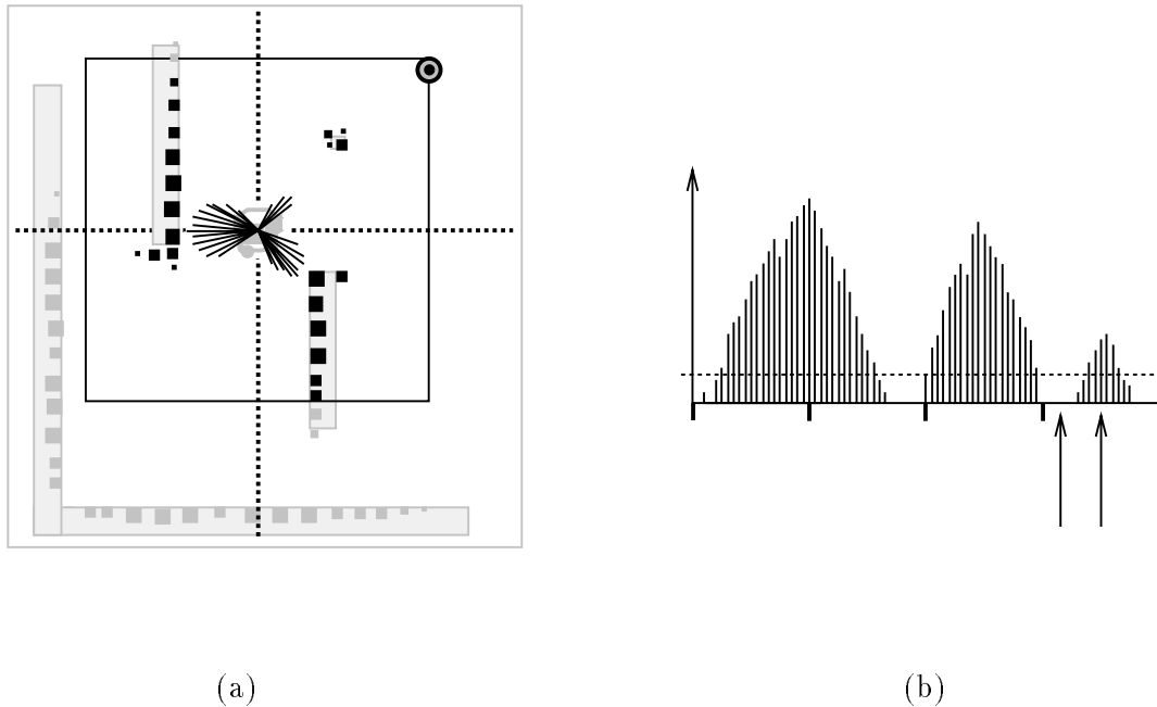
Figure 7: Using the data from the histogram grid in Figure 6b, CARMEL creates a second representation of objects called the polar histogram. In (a) above, histogram cells within the active window are used to form vectors centered at CARMEL; longer vectors represent objects that are nearer and more certain. In (b), these same vectors are represented in the polar histogram, which resembles a series of mountains and valleys. The target location is at 315 degrees relative to CARMEL's current location, but CARMEL will travel at 290 degrees — the valley indicates that this is a safe direction to travel. In (a), this means that CARMEL will pass between obstacles A and C on its way to the target, rather than between obstacles A and B.
