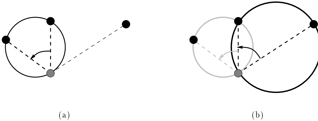
Figure 15: Three-object triangulation can be used to recalibrate the robot’s position when dead-reckoning errors have accumulated. To use this method, the locations of three objects A, B, and C are known, and the directions to the three objects from the perspective of the robot are known; the robot’s location is unknown. In (a), objects A and B, plus the angle between them (relative to the robot) are used to calculate a circle; the robot is somewhere on the perimeter of this circle, but its exact location is not yet known. In (b), a second circle is similarly calculated, using objects B and C. The two circles intersect at two points: the location of object B and the location of the robot.
