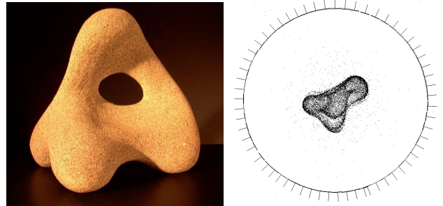
Figure 2: Reconstruction from the turntable sequence 'Stone'. No prior knowledge about the motion or the fact that it closes on itself was used in the estimation. The circular shape of the estimated trajectory is a verification of the correctness of the result. This result was obtained without any global bundle adjustment and exhibits a regularity and accuracy that is typically not obtained with an uncalibrated method until the calibration constraints have been enforced through bundle adjustment.
