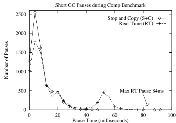
Figure 5: Compiler Benchmark (N=0.2Mb, O=1Mb)
