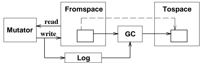
Figure 2: Replication and The Mutation Log
