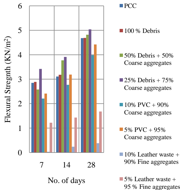
Fig.2. Variation of flexural strength in \text{KN/m}^2 with age of concrete in days
