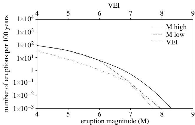
Figure 3. Graph showing numbers of eruptions per 100 years (on log scale) plotted against eruption magnitude (M) and Volcanic Explosivity Index (VEI). Two curves for magnitude 7 and above show current estimates of upper and lower expected numbers of very large eruptions, from analysis by Mason et al. (2004). VEI values from Decker (1990) based on volume of pyroclastic deposits. Very large events are rare; M7, one every 200 to 1000 years; M8, one every few tens of thousands of years or longer.
