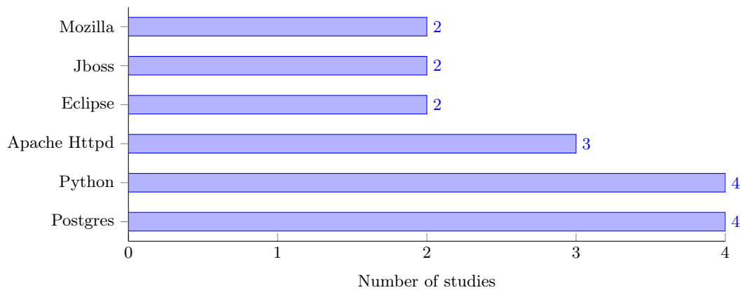
Figure 5: Projects most analyzed and the number of studies that used them as objects of study.
