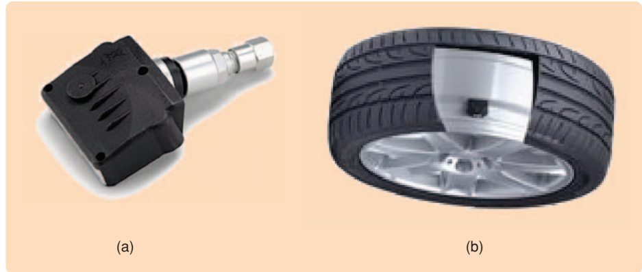
FIGURE 2 (a) Sensor module and (b) its fitting. The mass of the sensor is minimized to reduce the effect of centrifugal force due to rotation of the tire. The pressure sensor is mounted on the tire rim. The valve stem acts as an antenna for the built-in transmitter. (Printed with the permission of Hella, Inc.)
