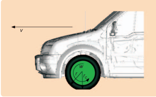
FIGURE 5 Tire and vehicle speeds. Tire pressure changes result in changes in tire rotational speed. Tire rotational speeds are measured in all vehicles by the antilock braking system.
