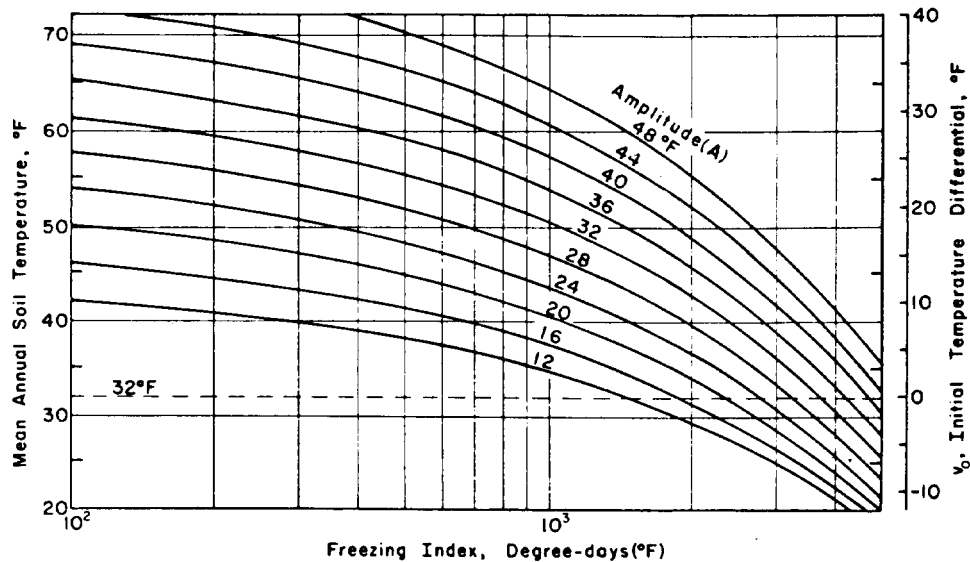
Figure D-1. Equivalent Sinusoidal Surface Temperature Amplitude A and Initial Temperature Difference V_o .
