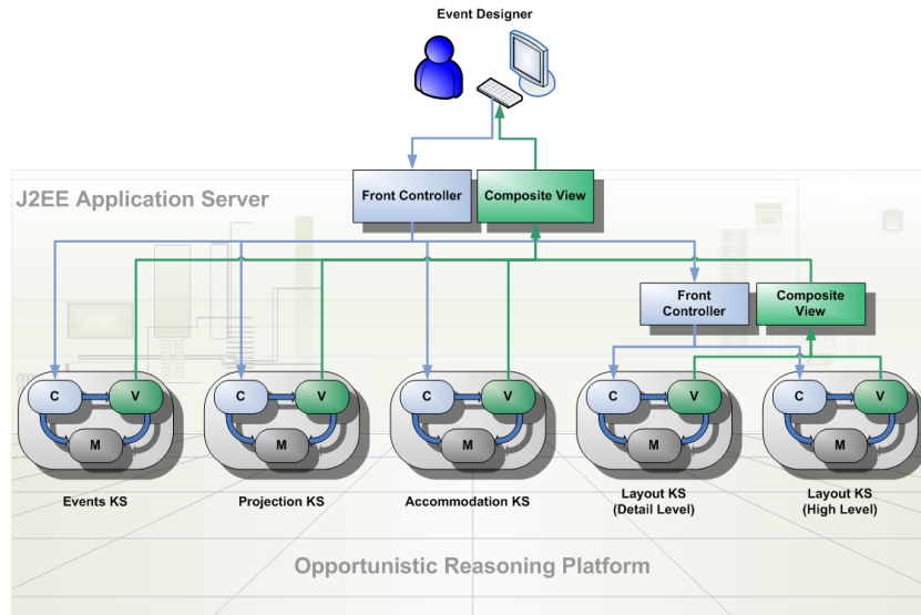
Fig. 4. ODEA deployed on a J2EE application server.
