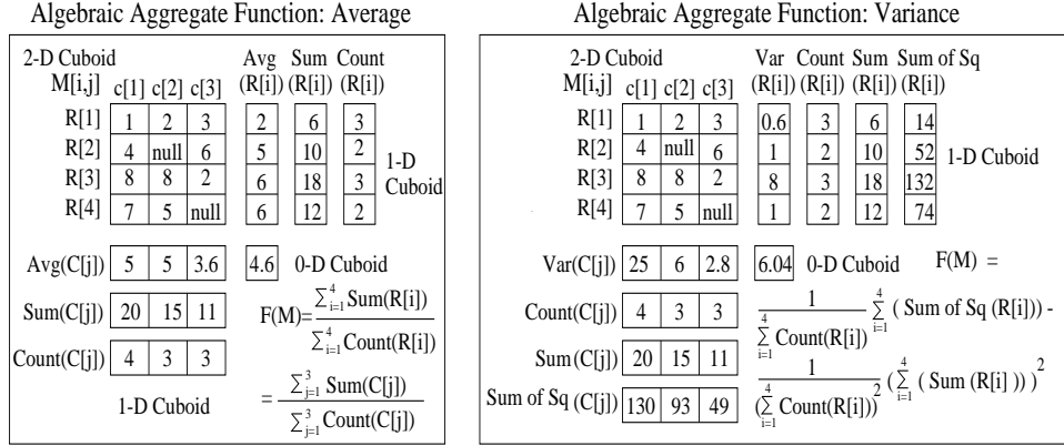
Figure 3: Computation of algebraic aggregate function
