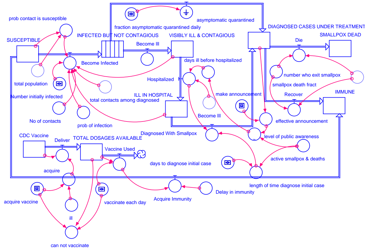
Figure 14: Bioterrorism Model
