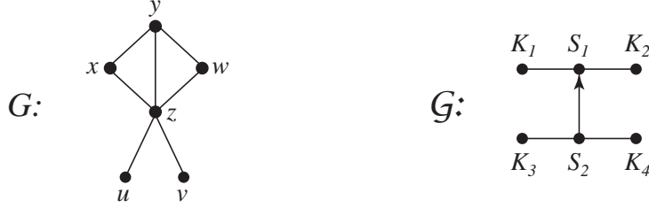
Figure 1: A chordal graph G and its clique-separator graph \mathcal{G} .
