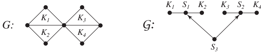
Figure 6: A chordal graph G and its clique-separator graph \mathcal{G} .
