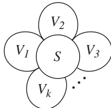
Figure 4: Chordal graph G .
