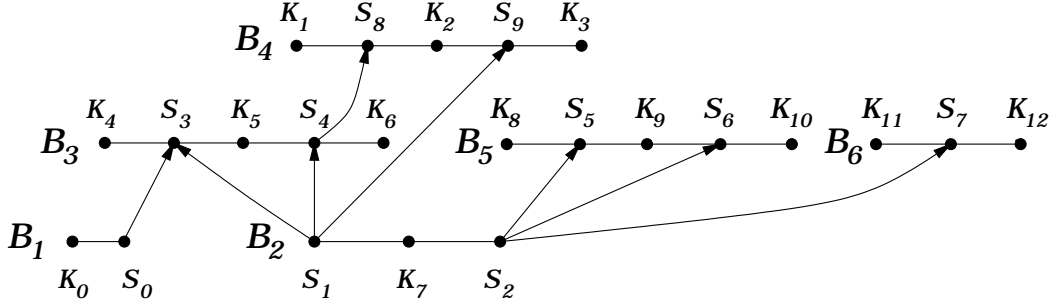
Figure 3: The clique-separator graph \mathcal{G} of the chordal graph in Figure 2.
