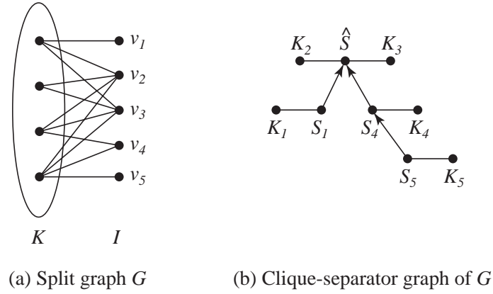
Figure 12: Example of Theorem 11-2.
