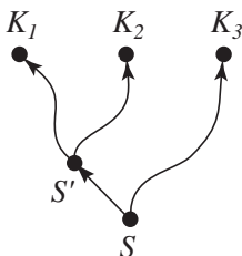
Figure 8: Proof of Theorem 8.
