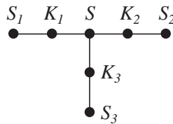
Figure 7: A separator node S with three neighbors that are internal nodes.
