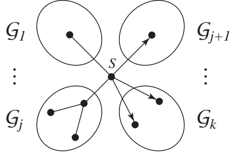
Figure 5: Clique-separator graph \mathcal{G} .
