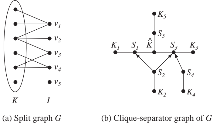
Figure 11: Example of Theorem 11-1.
