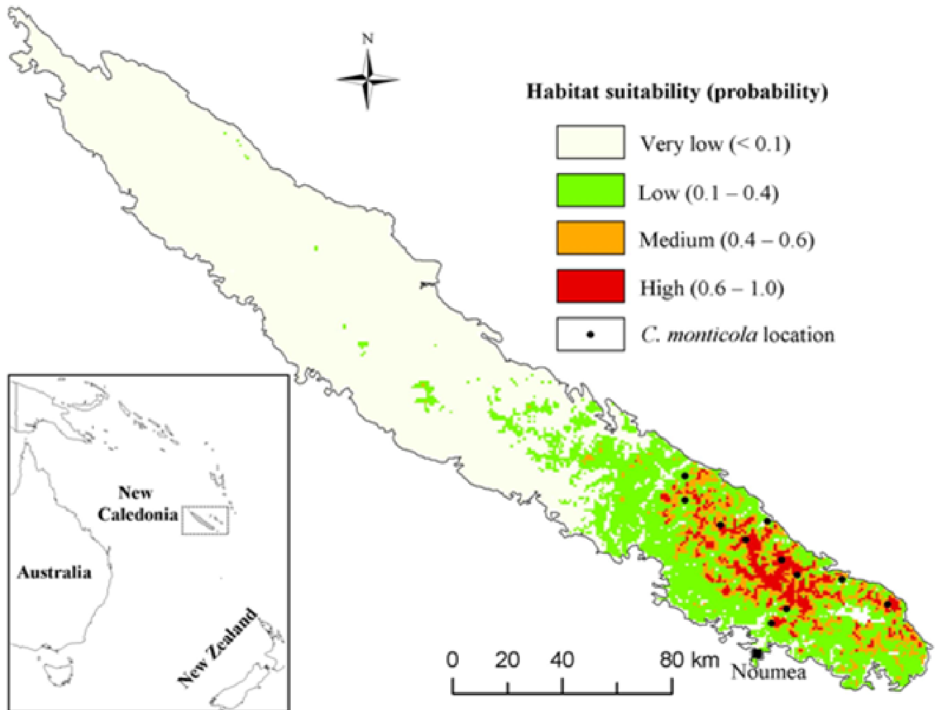
Figure 1. Predicted potential suitable habitat for C. monticola tree species on Grande Terre, the main island of New Caledonia.
