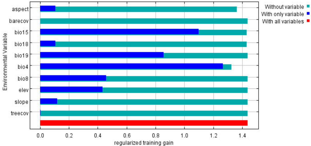
Figure 2. Results of jackknife evaluations of relative importance of predictor variables for C. monticola Maxent model. Note: 'elev' is elevation; 'barecov' and 'treecov' are MODIS percent bare cover and tree cover; 'bio 4' is temperature seasonality, 'bio8' is mean temperature of wettest quarter, 'bio15' is precipitation seasonality, 'bio18' is precipitation of warmest quarter, and 'bio19' is precipitation of coldest quarter.
