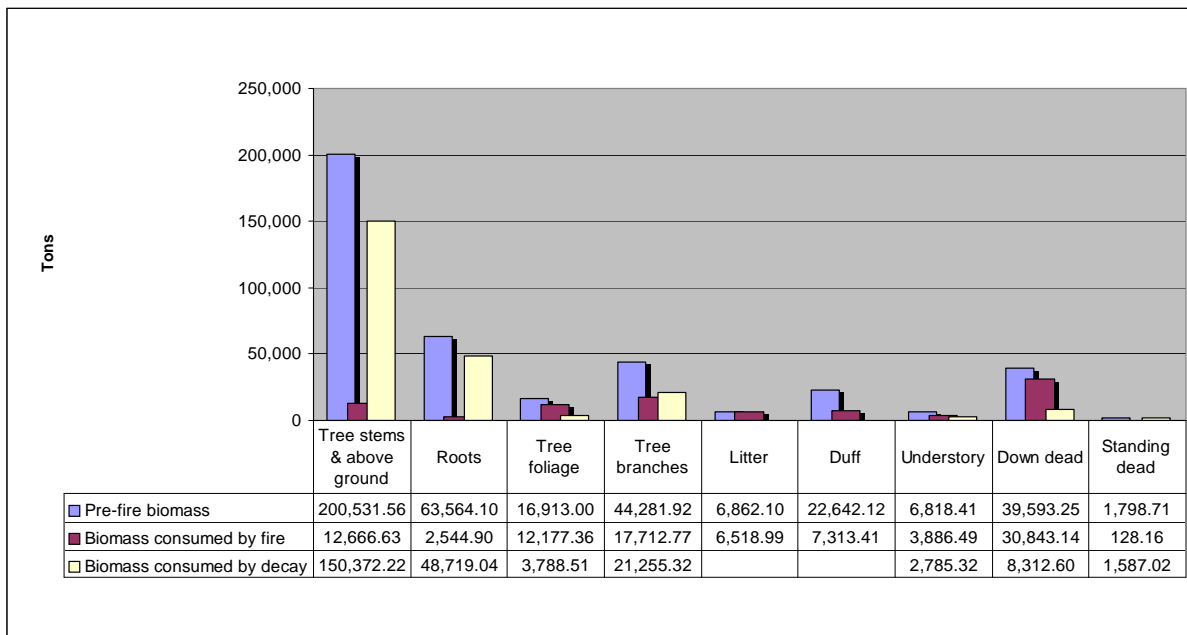
Figure 1. FCEM estimates of pre-fire biomass and biomass consumed by combustion and post-fire decay by forest component in the forest burned by the Angora Fire.
