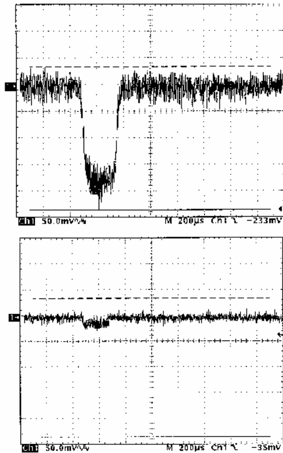
Figure 4 - A Li-ion battery with a 2A pulse current load (top), and same load with a 7F, 5mΩ capacitor in parallel (bottom) [9].
