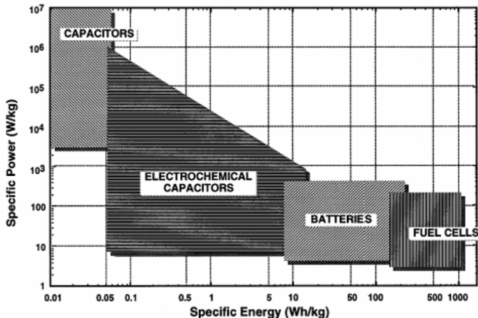
Figure 3 - Ragone plot for various energy storage devices [8].
