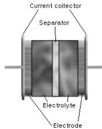
Figure 2 - EDLC cell composition.
