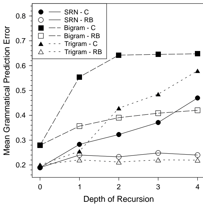
Cross-Dependency Recursion
