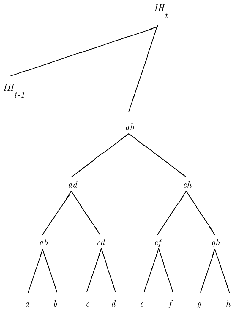
Figure 1: 8-leaf tree for the example of §3.
