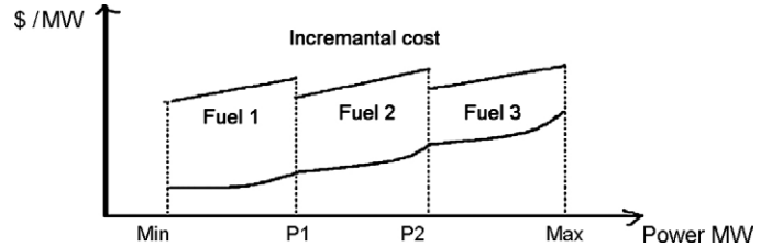
Fig. 2. Piecewise quadratic and incremental fuel cost function.
