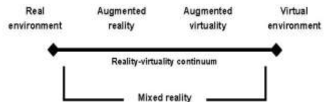
Fig. 1. Reality-virtuality continuum [107].
