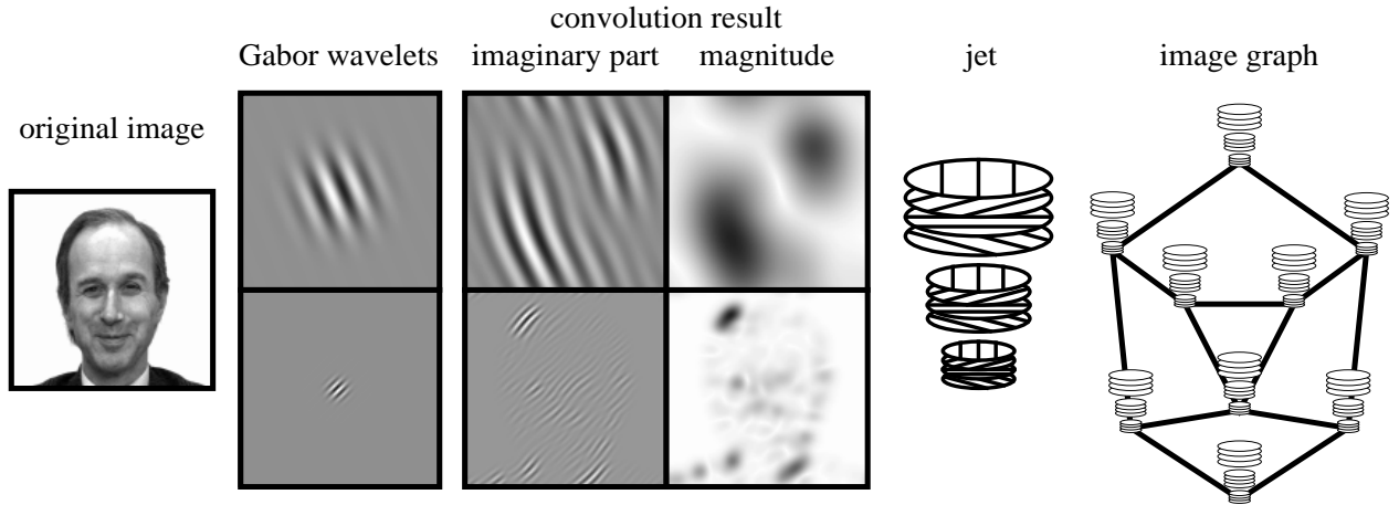
Figure 1: The graph representation of a face is based on the Gabor wavelet transform, a convolution with a set of wavelet kernels. These have the shape of plane waves restricted by a Gaussian envelope function. We compute 40 coefficients (5 frequencies \times 8 orientations). Coefficient phase varies approximately with wavelet frequency (see imaginary part), magnitude varies slowly. The set of 40 coefficients obtained for one image point is referred to as a jet (for clarity, only 3 frequencies and 4 orientations are represented in the figure). A sparse collection of such jets together with some information about their relative location constitutes an image graph, used to represent an object, such as a face.
