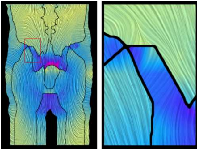
Figure 1: LIC image of a vector field (electrical field) containing discontinuities. Field strength |\mathbf{v}| is indicated by color.
