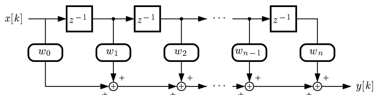
Figure 1: Structure of a linear, single-input single-output, FIR filter.
