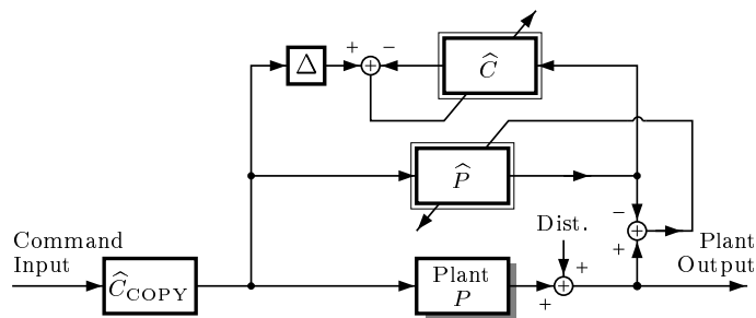
Figure 5: A system which is unbiased by disturbance.
