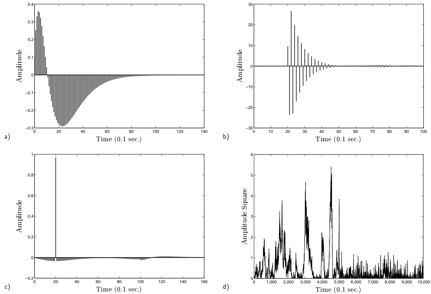
Figure 7: a) Impulse response of discretized stabilized nonminimum-phase plant; b) delayed inverse; c) convolution of plant impulse response with delayed-inverse impulse response; d) square of the output error, where disturbance cancelling began at the 5,000th sample time.
