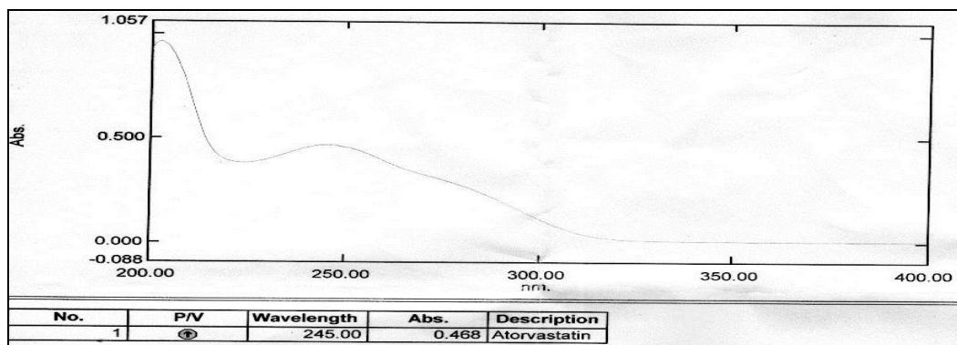
FIG: 3A UV SPECTRUM OF ATORVASTATIN IN DILUENT [Sample: Atorvastatin (10 µg/ml); Reference: Diluent]
