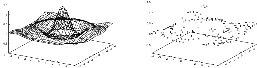
Figure 2: Approximation of f(x, y) = \text{sinc}\sqrt{x^2 + y^2} by two dimensional linear splines with accuracy \varepsilon = 0.01 (left) required 157 SV (right)
