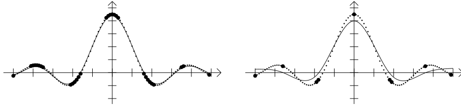
Figure 1: Approximations with different levels of accuracy require different numbers of SV: 31 SV for \varepsilon = 0.02 (left) and 9 SV for \varepsilon = 0.1 . Large dots indicate SVs.
