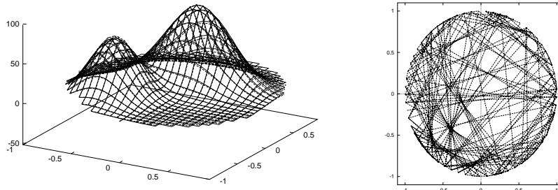
Figure 4: Original image (dashed line) and its reconstruction (solid line) from 2,048 observations (left). 172 SVs (support lines) were used in the reconstruction (right).
