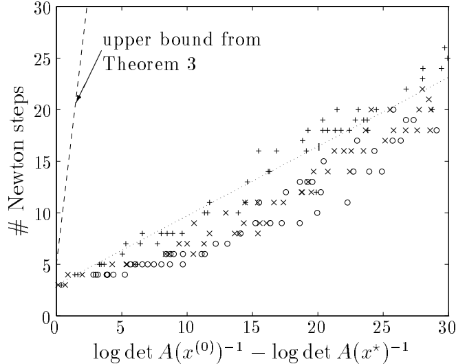
Figure 5: Number of Newton iterations to minimize \log \det A(x)^{-1} versus \log \det A(x^{(0)})^{-1} - \log \det A(x^*)^{-1} (with \delta = 2.33 \cdot 10^{-10} , i.e., \log_2 \log_2(1/\delta) = 5 ). Random matrix completion problems of three sizes ('+': m = 20 ; l = 20 , 'x': m = 20 , l = 100 , 'o': m = 50 , l = 100 ). The dotted line is a least-squares fit of the data and is given by 3 + 0.67(\log \det A(x^{(0)})^{-1} - \log \det A(x^*)^{-1}) . The dashed line is the upper bound of Theorem 3 ( 5 + 11(\log \det A(x^{(0)})^{-1} - \log \det A(x^*)^{-1}) ).
