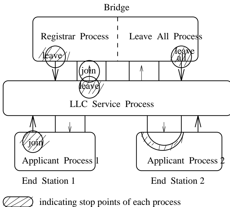
Figure 3: Deadlock in Non-Message-Overflow-Model
