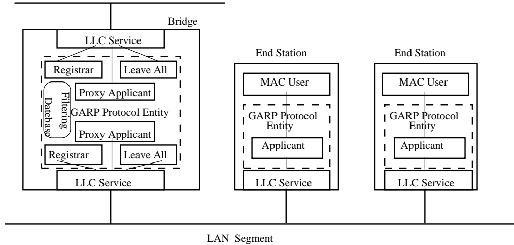
Figure 1: GARP Protocol Entity Components
