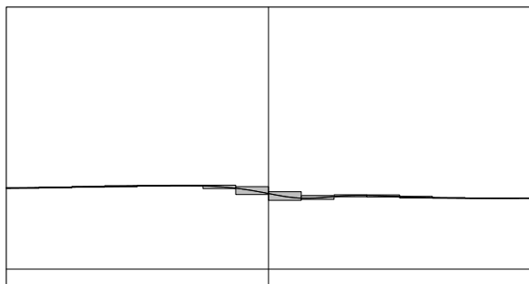
Figure 5: h(x) = g(g(x)) .
