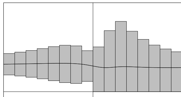
Figure 2: h(x) = g(g(x)) .
