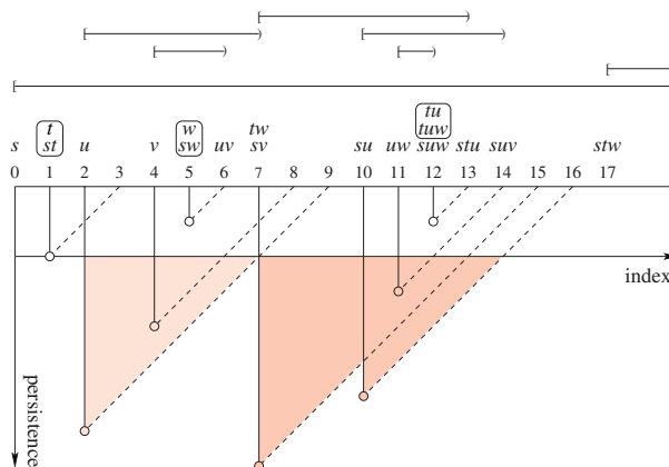
Fig. 10. The k -triangles that intersect the new axis at p = 2 have persistence 2 or larger. The simplex pairs representing cycles of persistence less than 2 are boxed.
