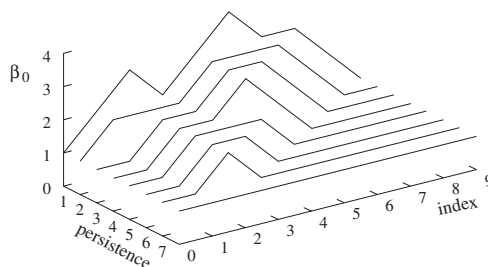
Fig. 11. Persistent 0th Betti numbers of the first ten complexes in the filtration of Fig. 3 and for persistence up to 7.
