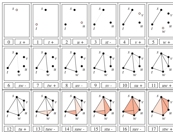
Fig. 3. The filter is the sequence of light simplices. The corresponding filtration is the sequence of complexes.
