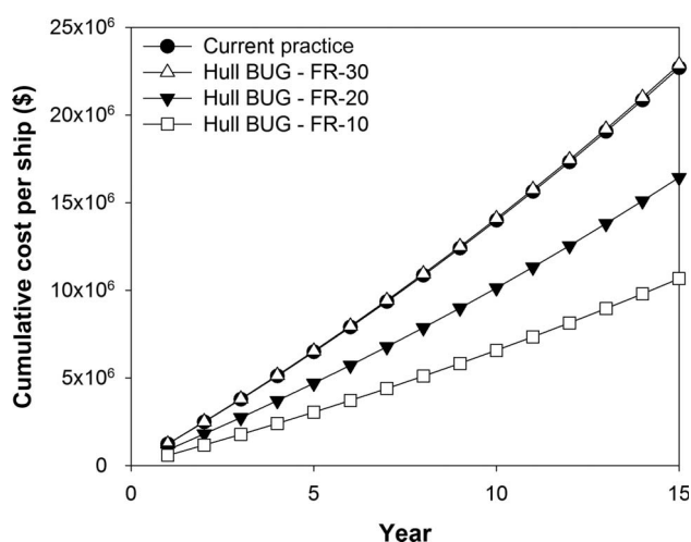
Figure 7. Cumulative costs (per ship) over 15 years for current hull coating and maintenance practices or maintenance using the Hull BUG strategy. Results for Hull BUG were calculated for three levels of efficacy (FR-10, FR-20, FR-30).
