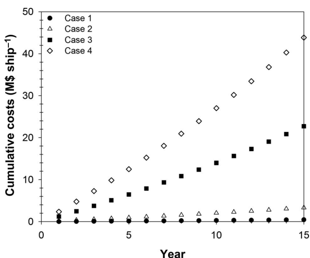
Figure 4. Cumulative costs (per ship) over 15 years resulting from coating roughness and fouling. See Table 5 for descriptions of the cases.
