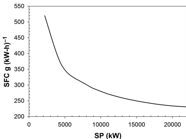
Figure 3. Specific fuel consumption (SFC) curve for the General Electric LM2500 gas-turbine engine adapted from Guimond et al. (2006).
