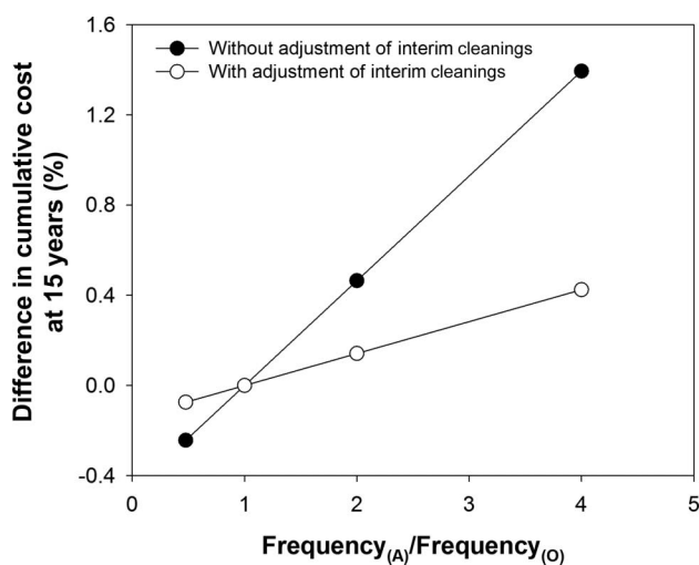
Figure 6. Effect of frequency of full hull cleanings on cumulative operating costs over 15 years. Variation in cleaning frequency is expressed as a multiple of the current mean frequency of full hull cleanings [ \text{Frequency}_{(O)} ]. Change in cumulative operating costs is expressed as a percentage of the cumulative costs assuming standard maintenance practices.
