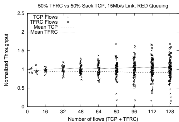
Figure 7: TCP competing with TRFC, with RED.
