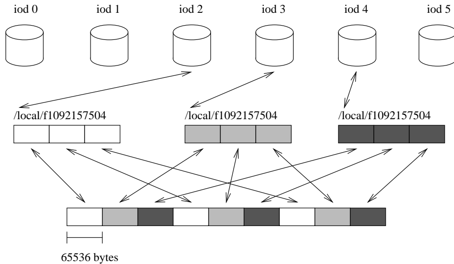
Figure 1: File-stripping example
