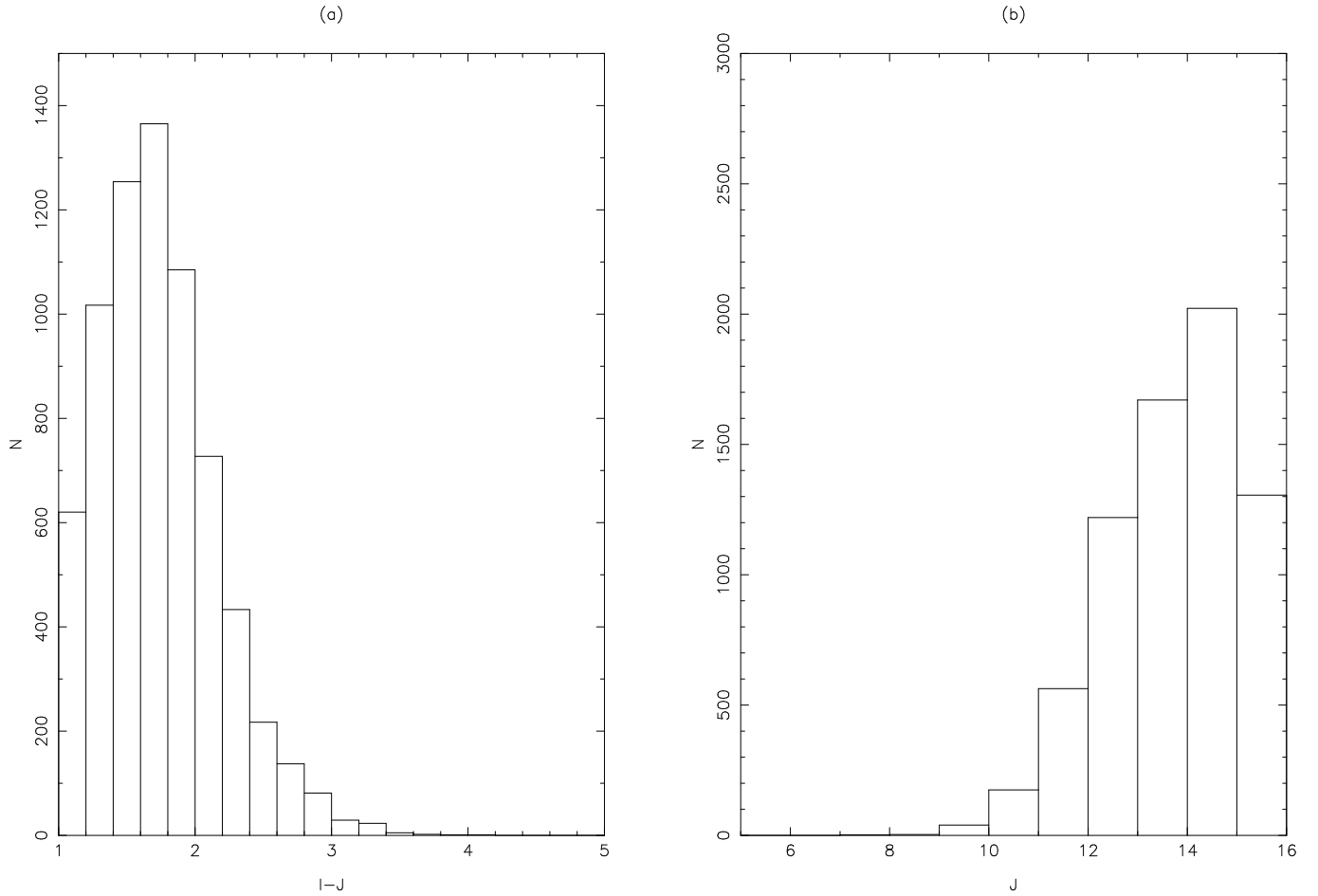
Fig. 2. Histograms showing the magnitude ( J ) and colour ( I - J ) of the objects found in this survey with proper motions between 0.1 and 0.5 arcseconds per year.
