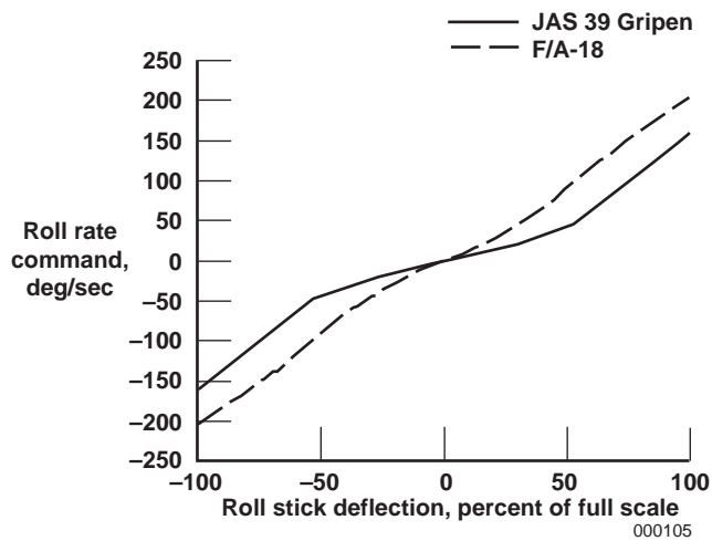
Figure 4. Comparison of stick gearing for roll commands for the Gripen and F/A-18.
