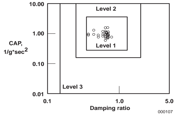
Figure 6. CAP analysis.
