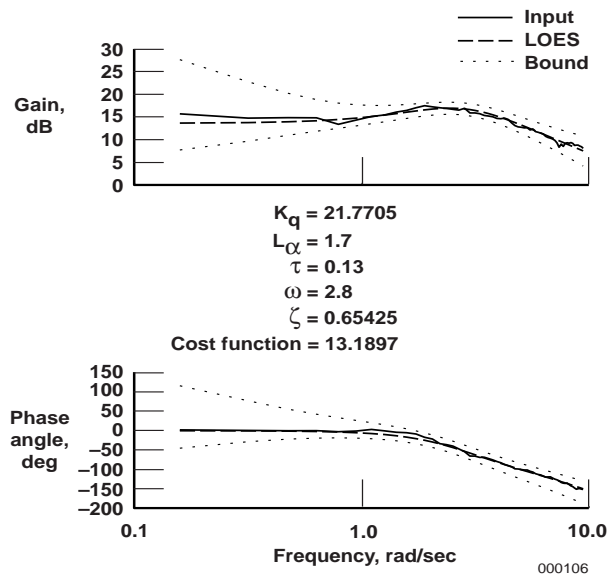
Figure 5. Typical LOES data fit of equation (1).
