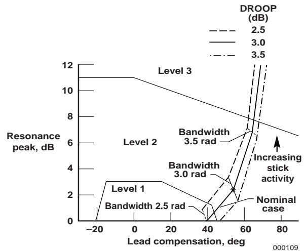
Figure 8. Neal-Smith carpet plot of representative case.
