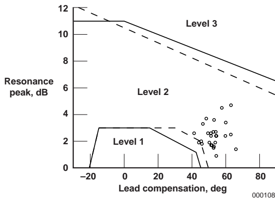
Figure 7. Neal-Smith analysis.
