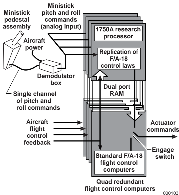
Figure 2. Engaged ministick system.
