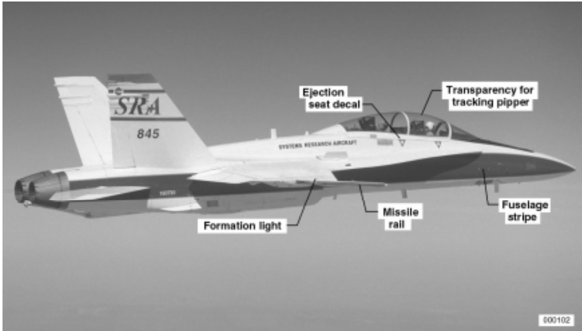
Figure 1. Systems Research Aircraft.
