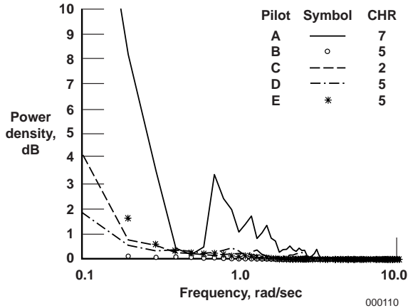
Figure 9. Power spectral density of echelon phase 3.
