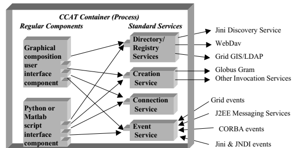
Fig. 1. Each CCAT Container process contains both user components and one instance of each of the Service Components. Many of the Service Components act as gateways to external wide-area services.
