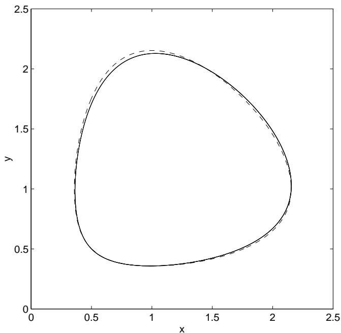
Figure 3: Cyclic solution with Modified Euler
