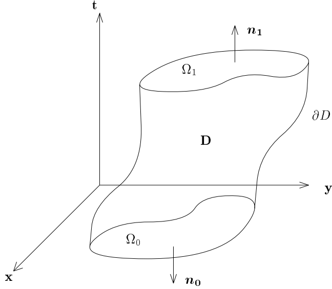
Figure 4: Area preserving mapping
