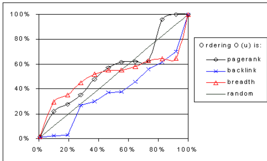
Graph 5. Percentage of DB group Web crawled vs. P_{ST}
